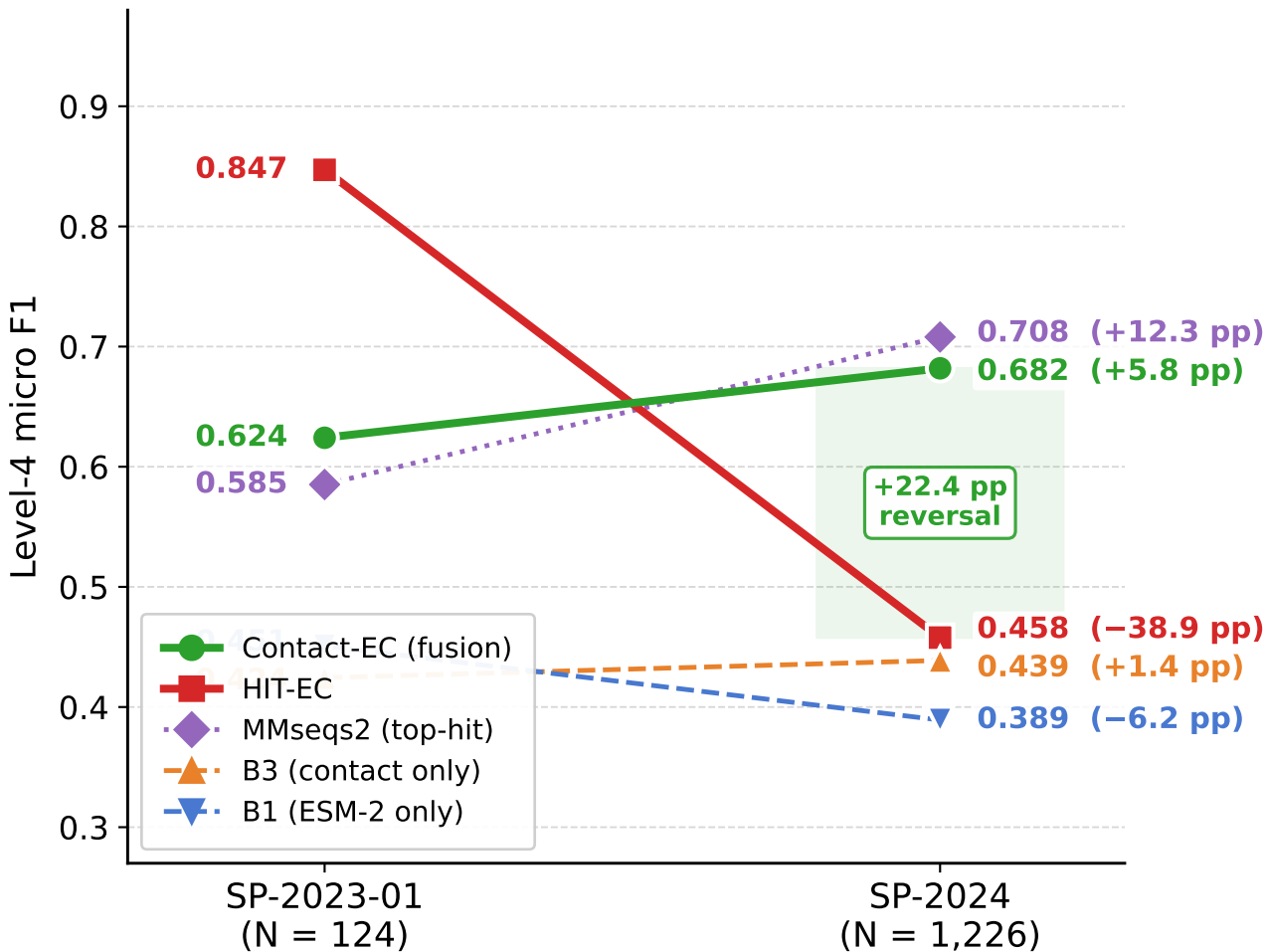
Model trajectories across temporal horizons
