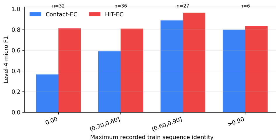
Figure 8: Level-4 micro F1 by maximum recorded train-set sequence identity on the 101 temporal proteins with available EC-Bench similarity metadata. The result motivates future Foldseek/TM-align or CATH/SCOP fold-disjoint testing.
