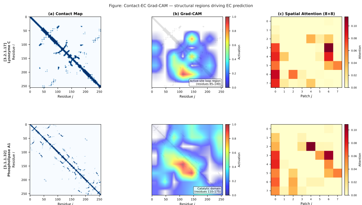
Figure 2: Grad-CAM structural interpretability for Contact-EC. Two correctly predicted test-set enzymes. (a) AlphaFold-derived contact map. (b) Grad-CAM heatmap overlaid on the contact map. (c) ResNet-50 spatial attention weights at the 8\times 8 feature-map level. Top : Lysozyme C (EC 3.2.1.17, UniProt C0HLB7). Bottom : Phospholipase A1 (EC 3.1.1.32, UniProt P0DPT0).
