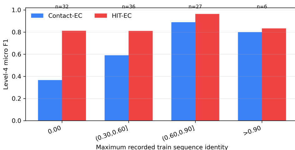
Figure 3: Level-4 micro F1 by maximum recorded train-set sequence identity on the 101 temporal proteins with available EC-Bench similarity metadata. The result motivates future Foldseek/TM-align or CATH/SCOP fold-disjoint testing.
