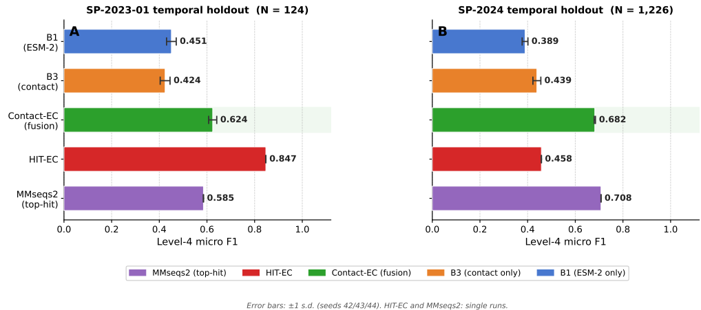
Figure 2 Level-4 micro F1 on two temporal holdouts. (A) SP-2023-01 ( N=124 ). (B) SP-2024 ( N=1,226 ). Error bars: \pm 1 s.d. across three training seeds (42/43/44); HIT-EC and MMseqs2 are single deterministic runs. Contact-EC is the only neural model that improves from Panel A to Panel B (+5.8 pp), while HIT-EC regresses -38.9 pp.
