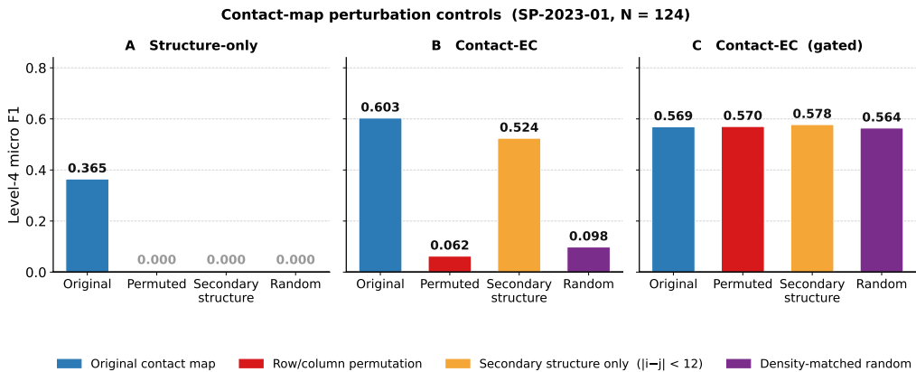
Figure 4 Contact-map perturbation controls (SP-2023-01, N=124 ), shown separately per model. (A) B3 (contact-map only) collapses to zero under all three perturbations, confirming reliance on genuine fold topology. (B) Contact-EC flat FC drops sharply under shuffling ( -54.1 pp) and density-matched random ( -50.5 pp) but retains most performance under diagonal-only ( -7.9 pp), indicating short-range secondary-structure contacts remain informative. (C) Contact-EC-Hier is invariant across all conditions ( \pm 1.0 pp), revealing that its gated cross-attention routes to the ESM-2 branch when topology is destroyed.
