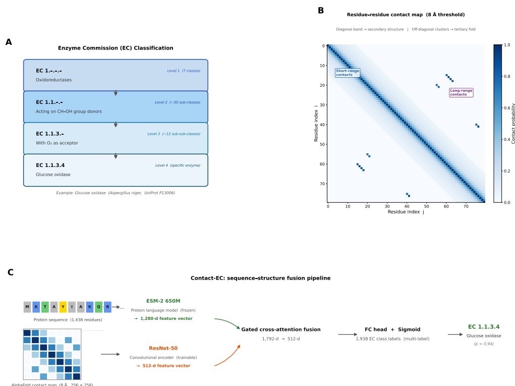
Figure 1 Contact-EC overview. (A) EC number four-level hierarchy illustrated with glucose oxidase (EC 1.1.3.4). (B) Example protein contact map (8 Å threshold); short-range backbone contacts form the diagonal band; long-range contacts (blue arrows) encode tertiary fold topology. (C) Contact-EC pipeline: ESM-2 (1280-d) and ResNet-50 contact-map encoder (512-d) are fused via gated cross-attention before a flat FC sigmoid head predicts all 1,938 Level-4 EC classes simultaneously.
