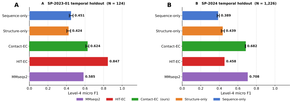
Figure 2 Level-4 micro F1 on two temporal holdouts. (A) SP-2023-01 ( N=124 ). (B) SP-2024 ( N=1,226 ). Error bars: \pm 1 s.d. across three training seeds (42/43/44); HIT-EC and MMseqs2 are single deterministic runs. Contact-EC is the only neural model that improves from Panel A to Panel B (+5.8 pp), while HIT-EC regresses -38.9 pp.
