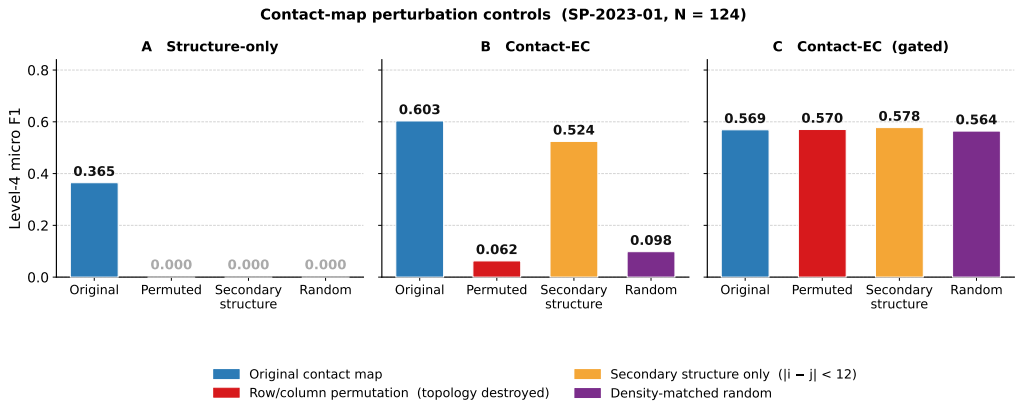
Figure 4 Contact-map perturbation controls (SP-2023-01, N=124 ), shown separately per model. (A) B3 (contact-map only) collapses to zero under all three perturbations, confirming reliance on genuine fold topology. (B) Contact-EC flat FC drops sharply under shuffling (−54.1 pp) and density-matched random (−50.5 pp) but retains most performance under diagonal-only (−7.9 pp), indicating short-range secondary-structure contacts remain informative. (C) Contact-EC-Hier is invariant across all conditions ( \pm 1.0 pp), revealing that its gated cross-attention routes to the ESM-2 branch when topology is destroyed.
