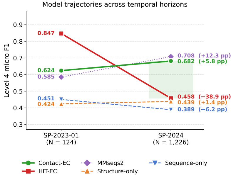
Figure 3 Model trajectories across the two temporal horizons. Each endpoint value and signed change (pp) is annotated in the model's colour. HIT-EC (red) falls -38.9 pp, whereas Contact-EC (green) improves +5.8 pp, producing a +22.4 pp reversal on SP-2024 (shaded region). Thick solid lines: our model and HIT-EC; thin dashed lines: single-modality baselines.
