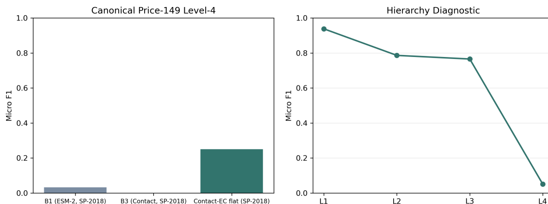
Figure S4: Price-149 failure analysis. Left: canonical Level-4 micro F1 for SP-2018 models. Right: hierarchical diagnostic for Contact-EC, showing that coarse EC levels remain predictable while exact Level-4 specificity collapses.
