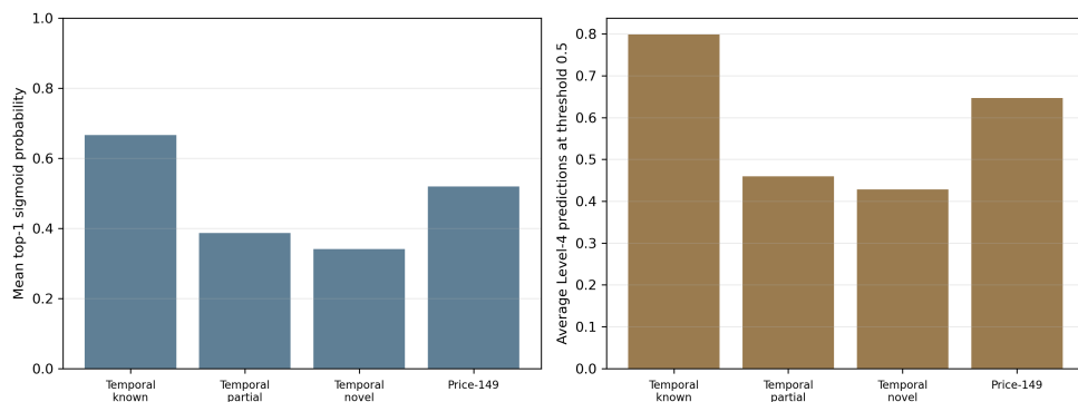
Figure S5: Contact-EC calibration and prediction-cardinality diagnostics. The audit separates empty prediction rate, average predicted-label cardinality, top-1 confidence, and top-1 correctness for temporal known, temporal partial, temporal novel, and Price-149 proteins.
