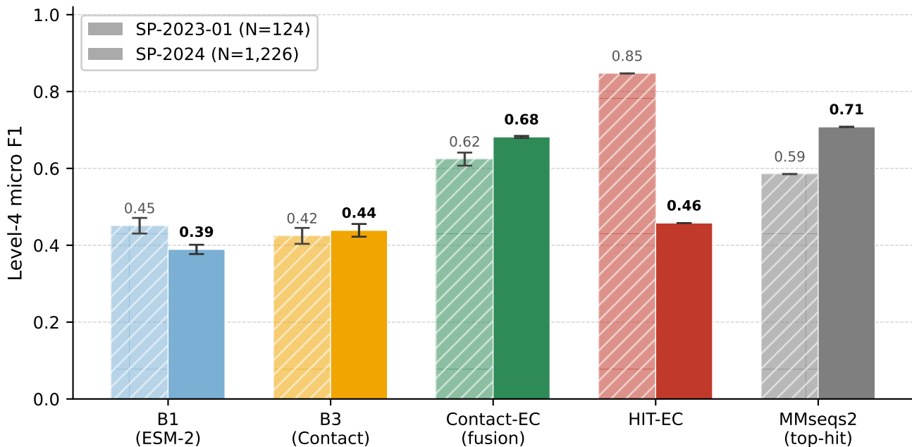
Temporal evaluation: SP-2023-01 vs SP-2024
