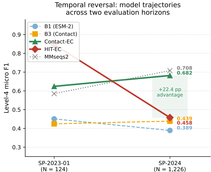
Figure 3 Model trajectories across evaluation horizons. HIT-EC falls -38.9 pp from SP-2023-01 to SP-2024, while Contact-EC improves +5.8 pp, yielding a +22.4 pp reversal. Dashed lines: single-modality baselines; solid lines: fusion and HIT-EC.
