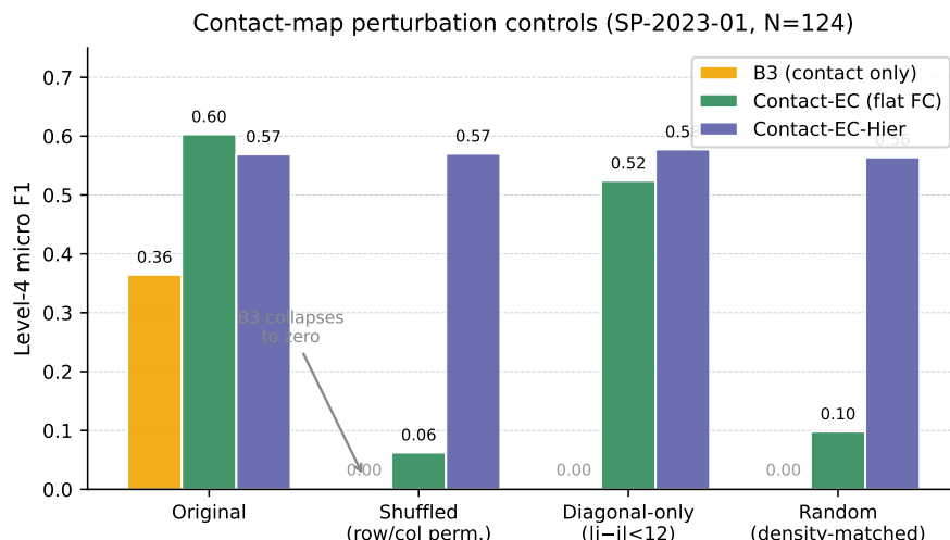
Figure 4 Contact-map perturbation controls on the SP-2023-01 temporal test ( N=124 ). B3 collapses to zero under all three perturbations, confirming reliance on genuine fold topology. Contact-EC flat FC drops sharply under shuffling and density-matched random maps but retains performance under diagonal-only maps (short-range contacts). Contact-EC-Hier is invariant, revealing that its gate routes to ESM-2 when topology is destroyed.
