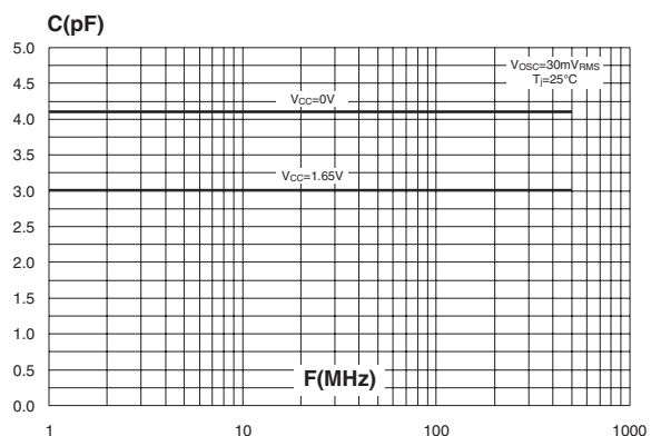
Figure 5: Frequency response
