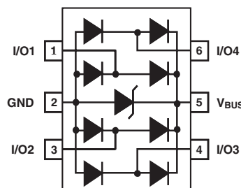
Figure 1: Functional Diagram
