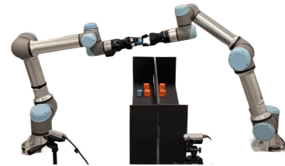
Fig. 1: Robotic manipulators performing an object handoff in a shelf stocking scenario [1].
