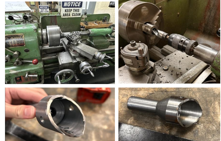
Manufacturing (Lathing & Angle Grinding)
