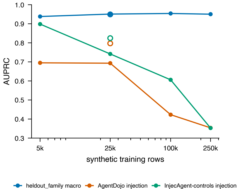
Figure 11: 2B LoRA at four v6-generator training sizes (5k–250k rows, single seed each; optimizer steps co-vary with rows) and one 2B full-parameter fine-tune at 25k rows (hollow markers). Held-out-family macro AUPRC is flat while AgentDojo and InjecAgent-controls injection AUPRC fall with more synthetic rows; full fine-tuning recovers most of the loss.
