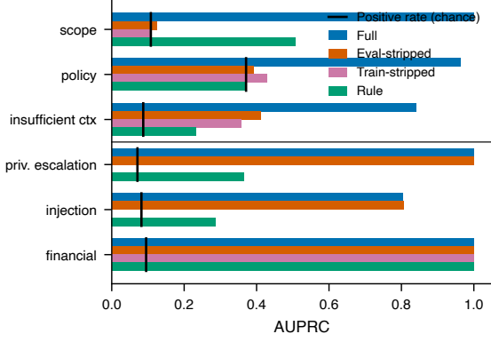
Figure 1: Decoder 2B v4, heldout_family: AUPRC per dimension with full input, identity removed at evaluation, identity removed at training, and the rule baseline; black ticks mark each dimension’s positive rate (chance). The top three dimensions are functions of the removed fields. v4 injection text carries the label leak of §8; its evidence sits in the call arguments, which stripping does not touch. Evaluable n and exact values in Table 8.
