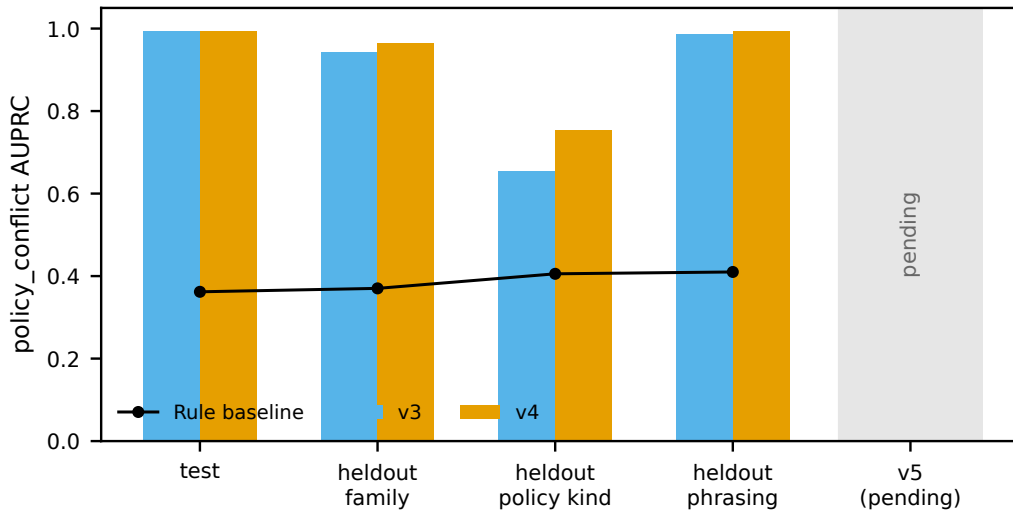
Figure 2: Decoder 2B, policy_conflict AUPRC across splits for the v3 and v4 generators (synthetic data; n per split matches Table 3), with the rule baseline’s policy_conflict AUPRC on each split shown as a line. The v5 slot is left blank pending that run. Source: docs/results/synthetic-v2/decoder-2b-v3/, decoder-2b-v4/.
