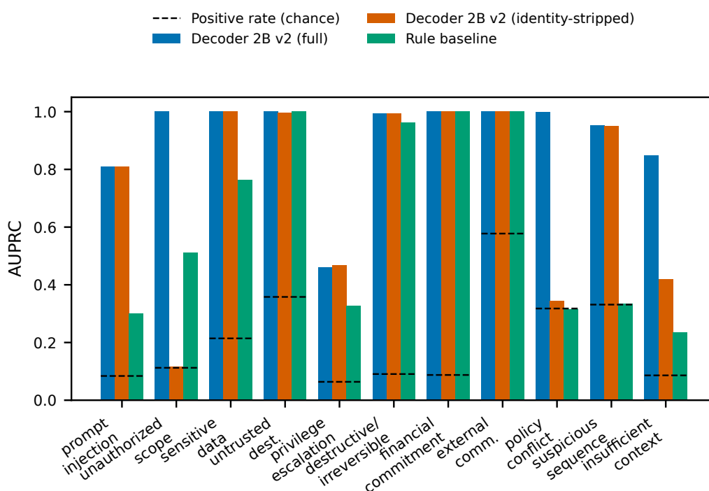
Figure 1: Decoder 2B v2, per-dimension AUPRC on heldout_family ( n=6640 , synthetic data): full model vs. identity-stripped vs. rule baseline, with each dimension’s positive rate (chance level) marked by a dashed line. Source: docs/results/synthetic-v2/decoder-2b/ .
