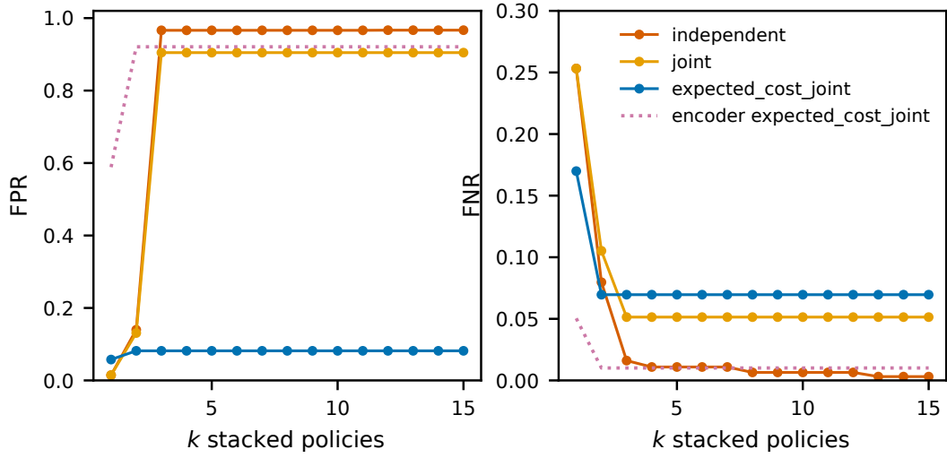
Figure 6: Decoder 2B, FPR (left) and FNR (right) vs. number of stacked policies k on heldout_family ( n=6640 ), for independent , joint , and expected_cost_joint strategies; the granite-embedding-r2 encoder’s expected_cost_joint curve is dotted. The independent step at k=3 is the fail-closed conservative bundle entering; the flat expected_cost lines follow from the covered set saturating at k=2 (§5).
