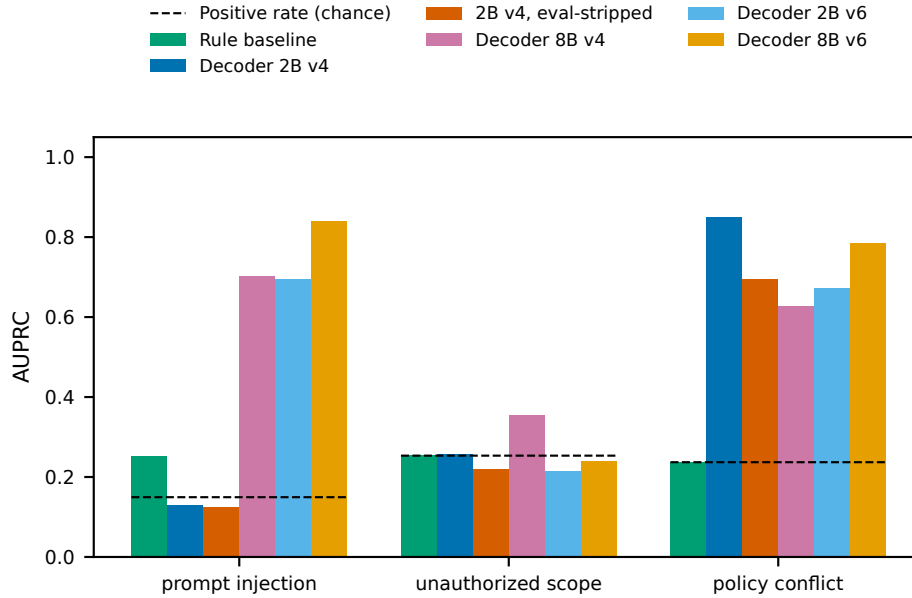
Figure 7: AUPRC on AgentDojo banking traces for the three learned dimensions: rule baseline, decoder 2B v4, 2B v4 eval-stripped, decoder 8B v4, and the leak-free 2B v6 and 8B v6, zero-shot, with each dimension’s positive rate as a dashed line.
