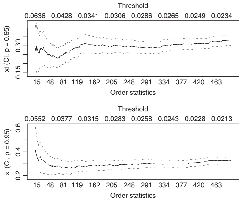
Figure 7.4 Scatterplots of Hill estimator for daily log returns of IBM stock. Sample period is from July 3, 1962, to December 31, 1998: upper plot is for positive returns and lower one for negative returns.
