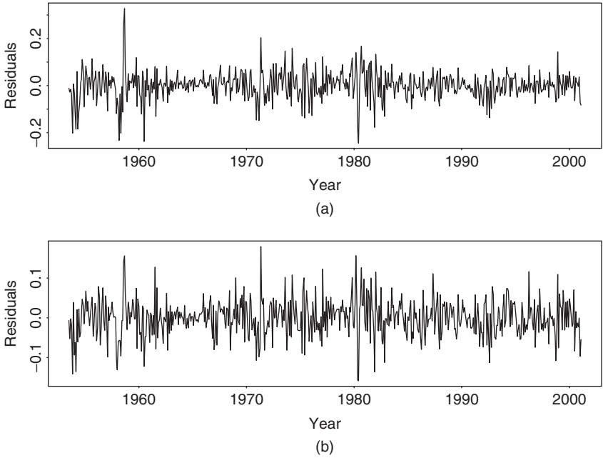
Figure 8.9 Residual plots for log U.S. monthly interest rate series of Example 8.6. Fitted model is VARMA(2,1): (a) 1-year rate and (b) 3-year rate.
