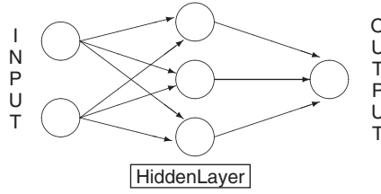
Figure 4.8 Feed-forward neural network with one hidden layer for univariate time series analysis.
