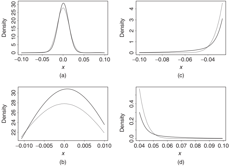
Figure 6.9 Density comparisons between normal distribution and distribution of Eq. (6.31). Dotted line denotes the normal distribution. Both distributions have mean zero and variance 2.0572 \times 10^{-4} . (a) Overall comparison, (b) comparison of peaks, (c) left tails, and (d) right tails.
