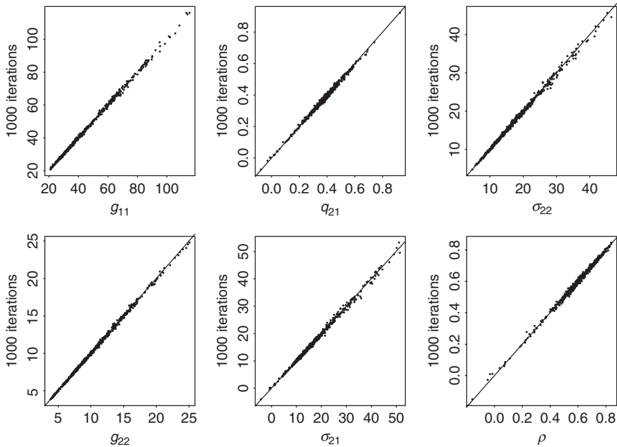
Figure 12.8 Scatterplots of posterior means of various statistics of two different Gibbs samples for bivariate stochastic volatility model for monthly log returns of IBM stock and S&P 500 index. The x axis denotes results based on 500 + 2000 iterations and the y axis denotes results based on 500 + 1000 iterations. Notation is defined in text.
