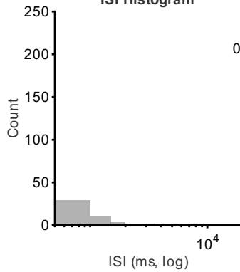
ISI Histogram
