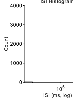
ISI Histogram
