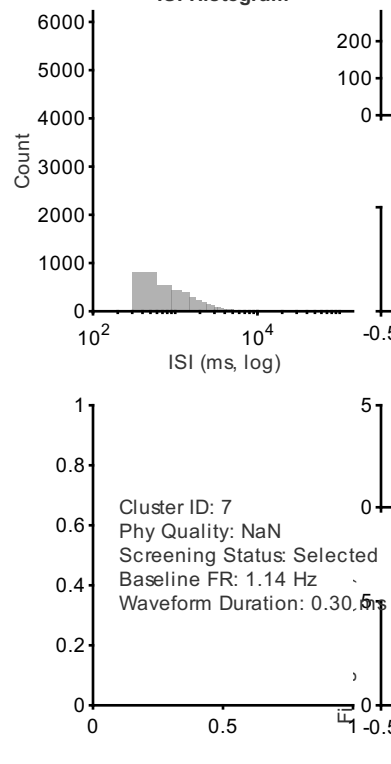
ISI Histogram
