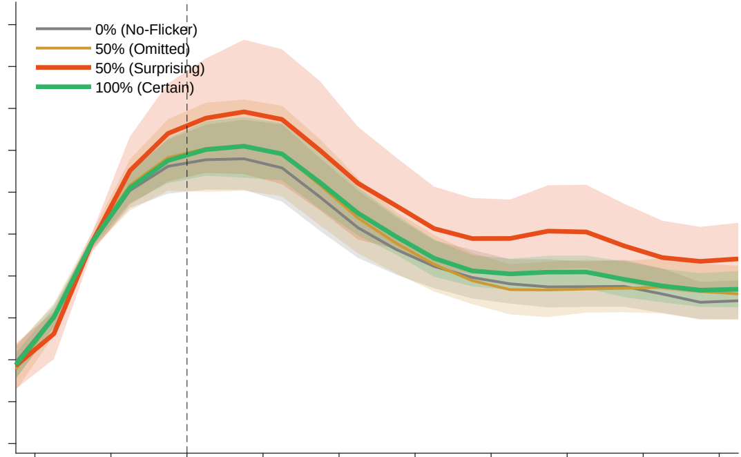
B. SPE: n=[60, 29, 27, 70]
