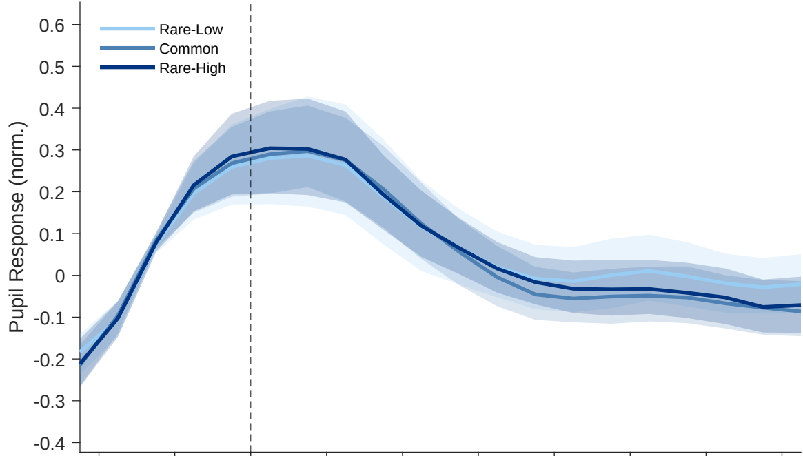
A. RPE (Normal Dist): n=[26, 30, 28]
