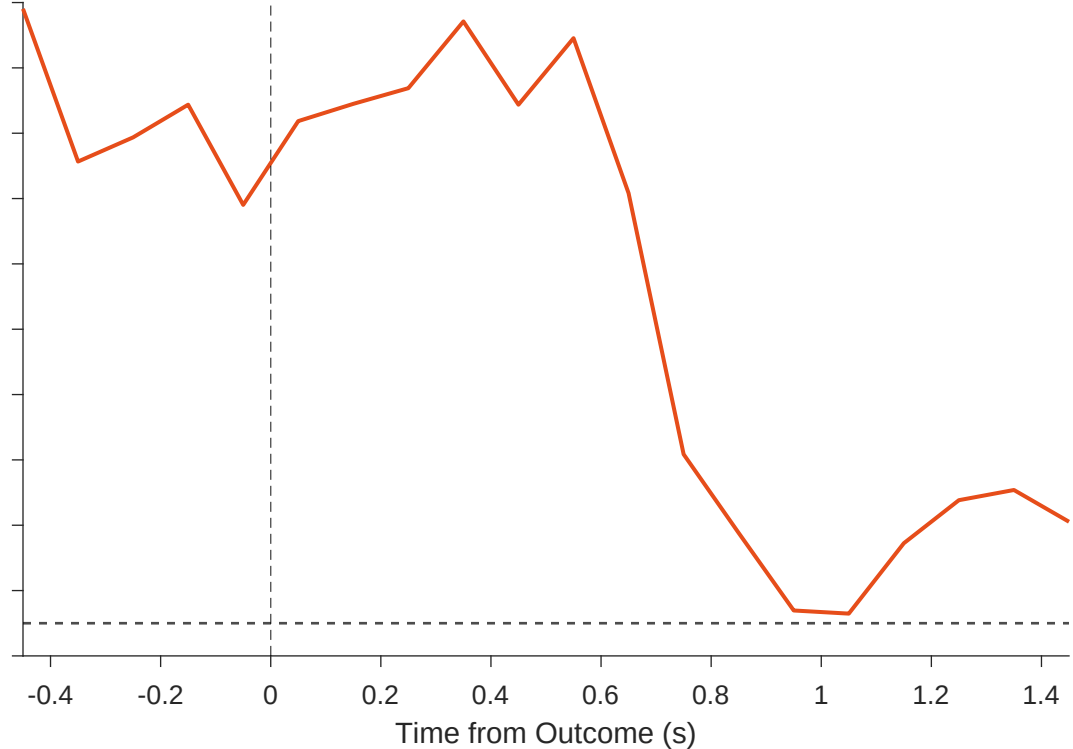
Surprising vs Certain (ranksum)
