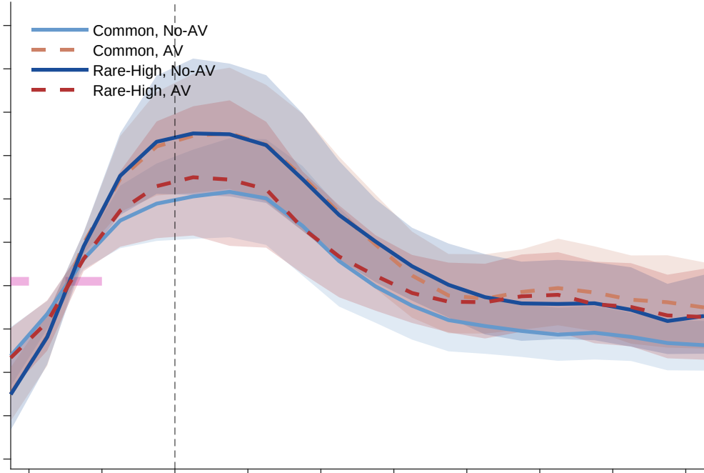
C. RPE x AV: n=[12,18; 15,13]
