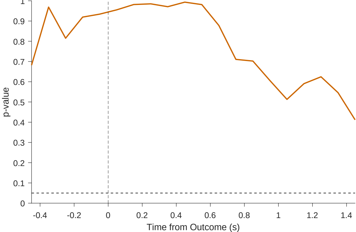
RPE Effect (1-way ANOVA)
