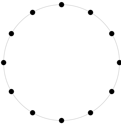
hop 3
