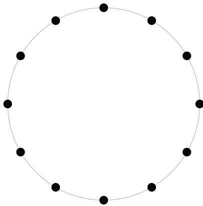
hop 2
