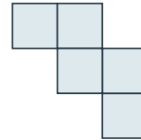
Stair: before 12; 0 or +2
