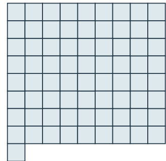
73 squares: 9 \times 8 plus 1; P = 36
