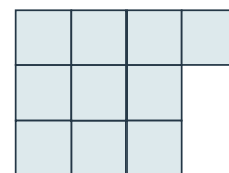
10 tiles: rows 4,3,3; P = 14
