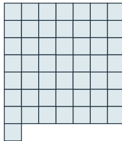
50 squares: 7 \times 7 plus 1; P = 30
