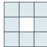
Frame: before 16; -4 or +2
