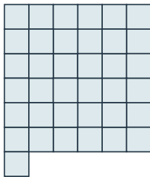
37 squares: 6 \times 6 plus 1; P = 26
