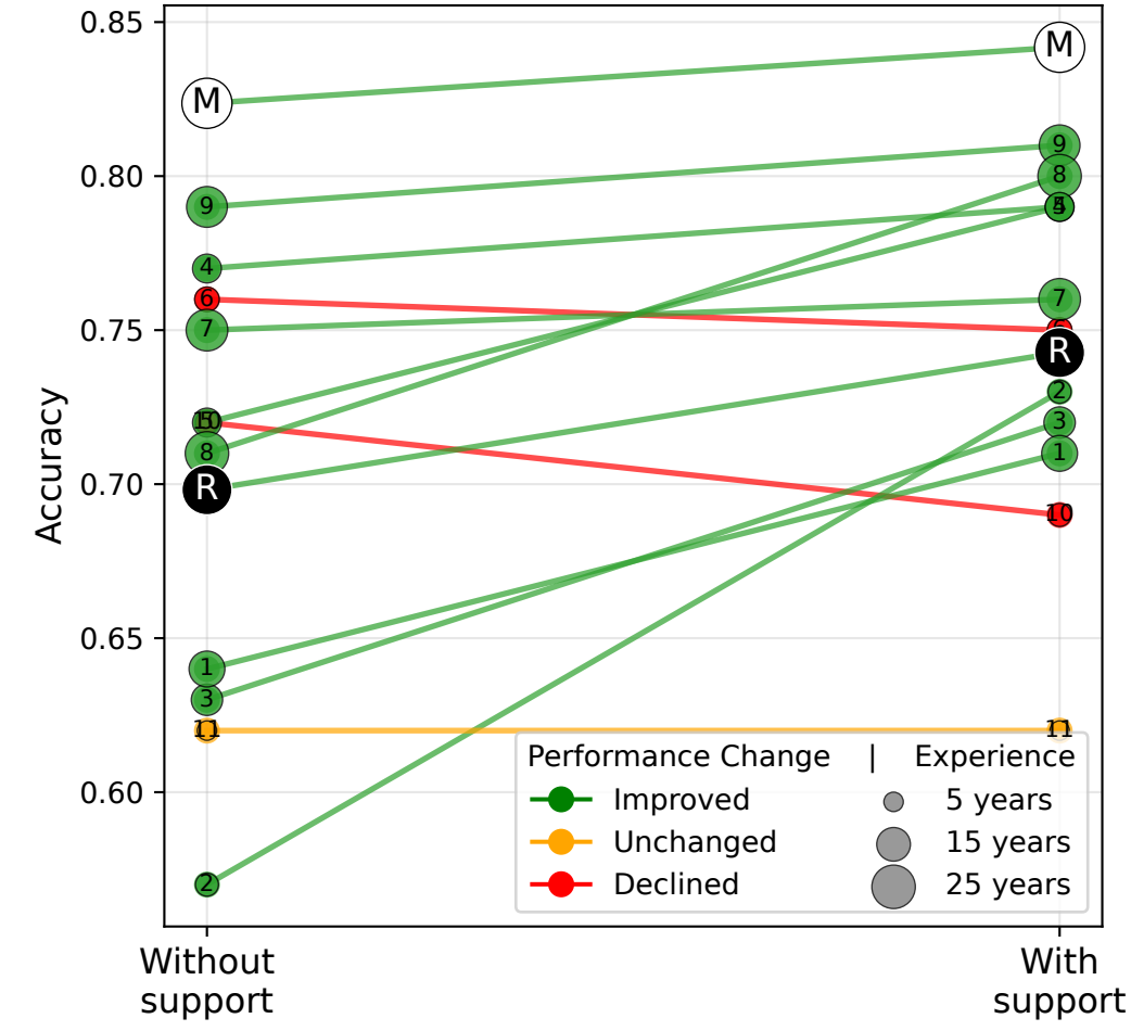
c) Individual agent performance change
