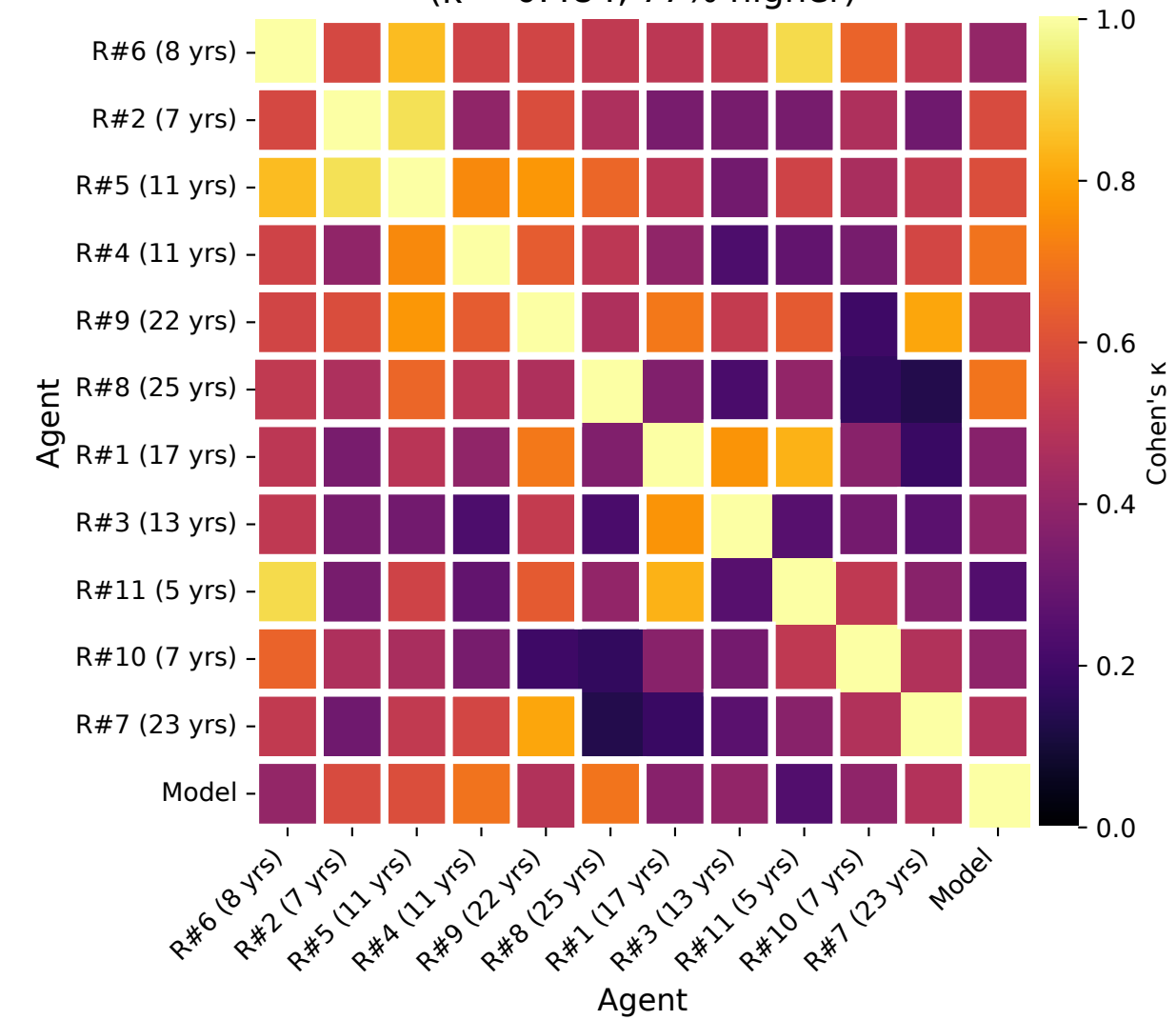
h) Inter-rater agreement with support ( \bar{\kappa} = 0.484 , 77% higher)
