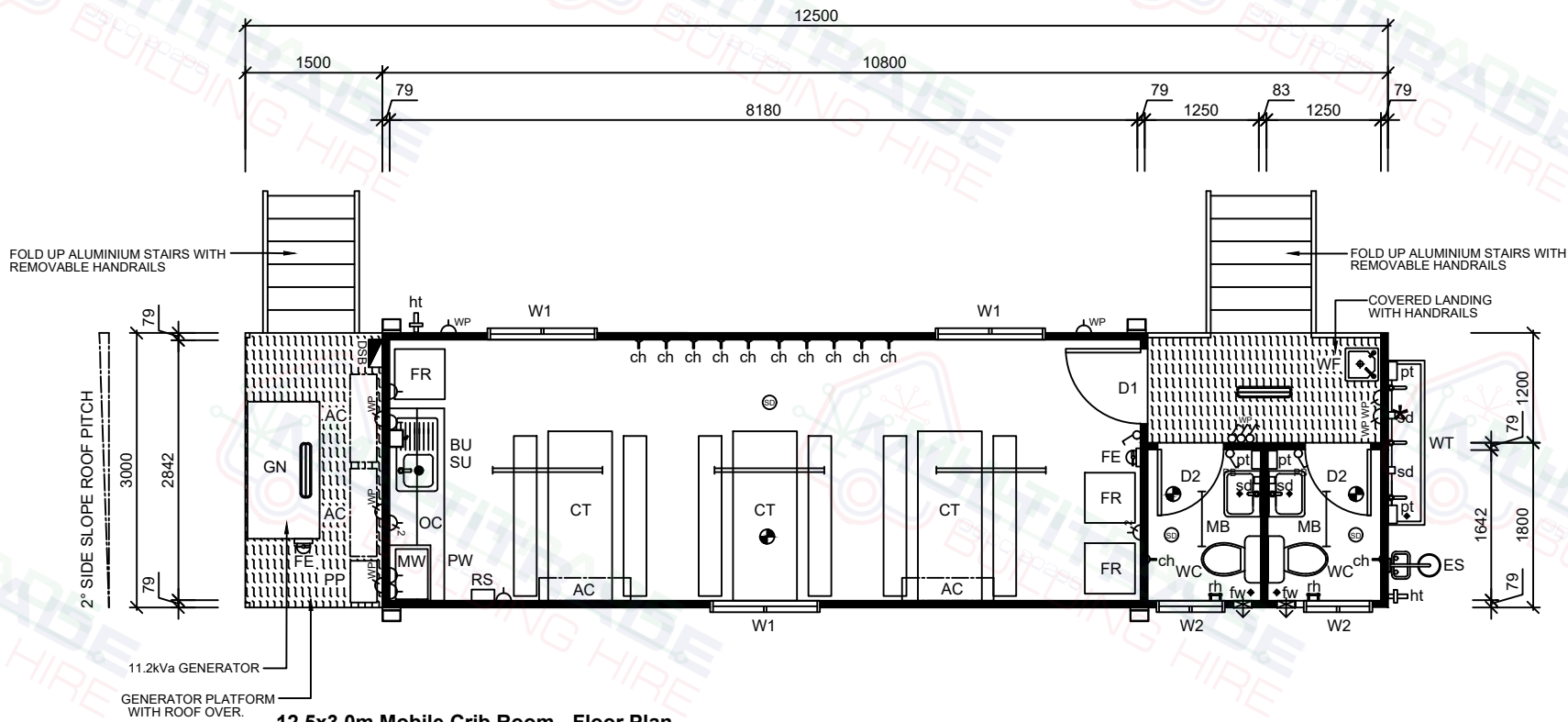
12.5x3.0m Mobile Crib Room - Floor Plan
