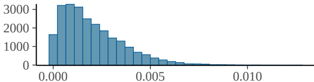
sd_study_id:arm__time_hours
