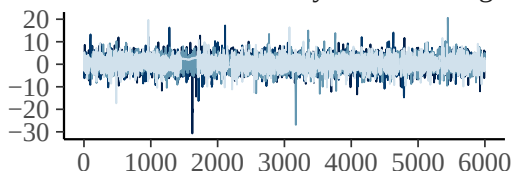
bs_stime_hours:recovery_modemassage_1
