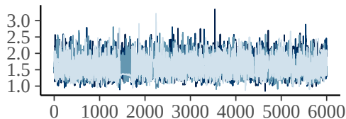
sd_study_id__Intercept
