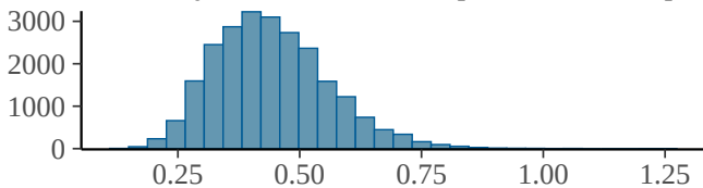
sd_study_id:arm:outcome_specific__Intercept
