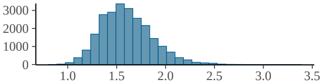
sd_study_id__Intercept
