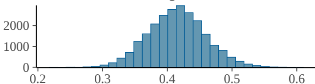
sigma
