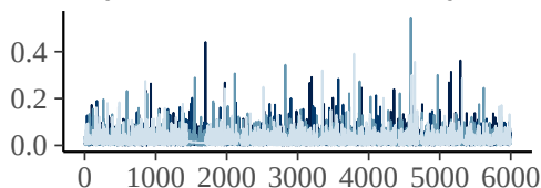
tudy_id__time_hours:recovery_moc
