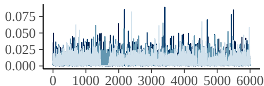
ly_id__time_hours:recovery_modep
