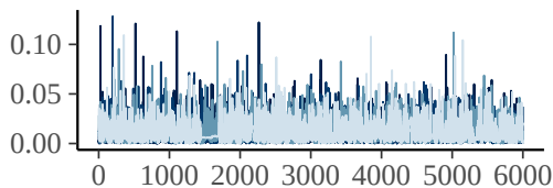
idy_id__time_hours:recovery_mode
