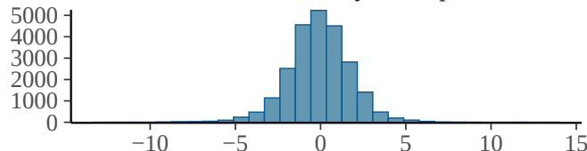
bs_stime_hours:recovery_modeplacebo_1
