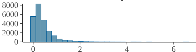
sds_stime_hoursrecovery_modecontrol_1
