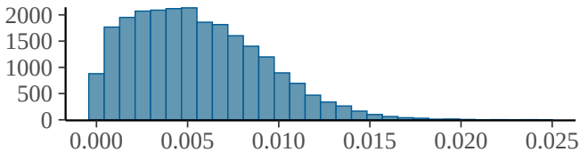
sd_study_id__time_hours
