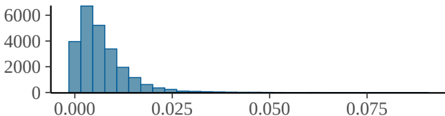
sd_study_id__time_hours:recovery_modeplacebc
