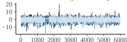
bs_stime_hours:recovery_modecompression_1
