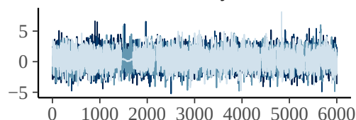
bs_stime_hours:recovery_modecontrol_1
