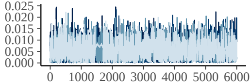
sd_study_id__time_hours
