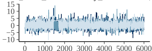
bs_stime_hours:recovery_modecontrast_1
