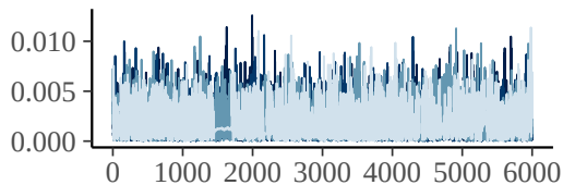
sd_study_id:arm__time_hours
