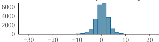
bs_stime_hours:recovery_modemassage_1
