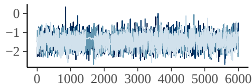
b_Intercept
