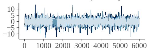
bs_stime_hours:recovery_modeplacebo_1
