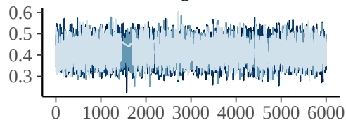
sigma
