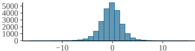
bs_stime_hours:recovery_modebfr_1
