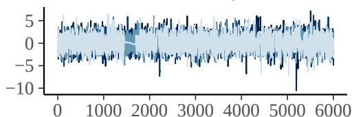
bs_stime_hours:recovery_modecold_1
