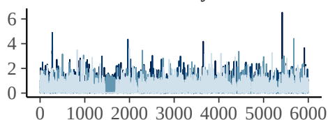
sds_stime_hoursrecovery_modecontrol
