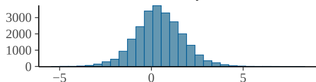
bs_stime_hours:recovery_modecontrol_1
