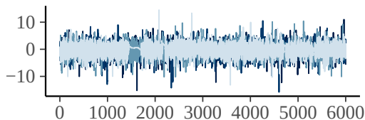
bs_stime_hours:recovery_modebfr_1
