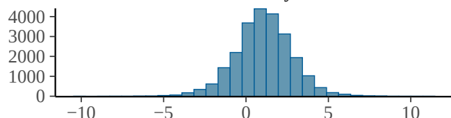
bs_stime_hours:recovery_modeactive_1
