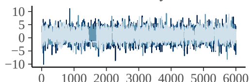
bs_stime_hours:recovery_modeactive_1
