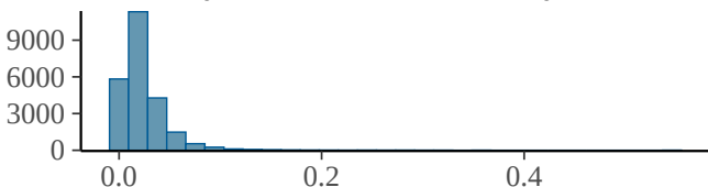
sd_study_id__time_hours:recovery_modebfr
