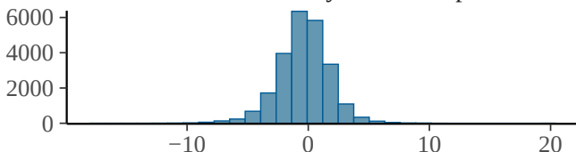
bs_stime_hours:recovery_modecompression_1
