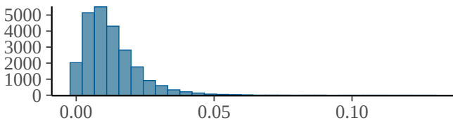
sd_study_id__time_hours:recovery_modeactive
