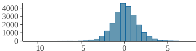
bs_stime_hours:recovery_modecold_1
