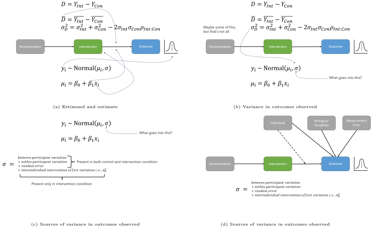
Figure 2: Mapping of estimand and estimate in the randomised controlled trial design for estimating average intervention effects alongside the directed acyclic graph. In (a) we have defined the estimand of the average treatment effect, our estimate based on the marginal distributions of interventions and controls (i.e., the causal arrow from intervention to outcome), and the standard deviation of treatment effects in addition to the general linear model estimator used to yield and estimate of this average treatment effect. The components of the general linear model are mapped to their corresponding components in the causal structure including the observed outcomes y_i , the randomly assigned intervention x_i , and the estimated average causal effect of the intervention compared to the control \beta_1 . In (b), (c), and (d) it shows that some of the variance in observed outcomes i.e., \sigma , may be due to intervention effect heterogeneity i.e., \sigma_D^2 (the dashed arrow in (d) depicting interaction of the individual with the intervention), but that there are numerous other sources of variance and that these also differ between the intervention and control conditions.
