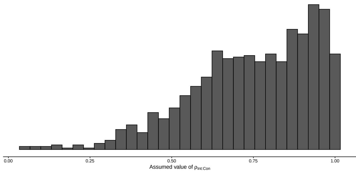
Figure 4: Histogram of the assumed values of \rho_{Int:Con} for each variance contrast in the dataset.
