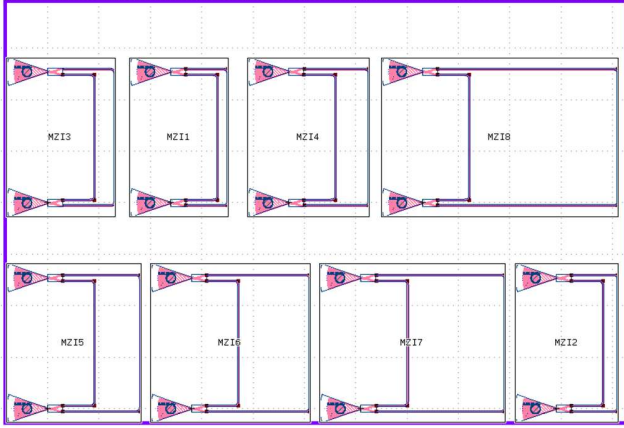
Fig 9. Layout for fabrication consisting of 8 MZIs
