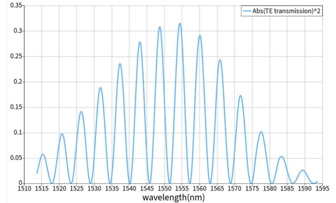
Fig 7. Transmission of MZI with two grating couplers
