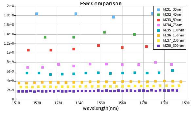
Fig 10. A comparison and sanity check for validity of FSR readings between 1 to 20nm
