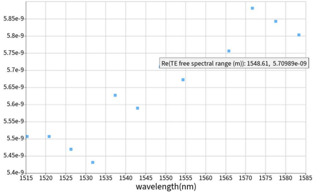
Fig 8. Free Spectral Range vs Wavelength of MZI with a pathlength difference of 100\mu\text{m} as seen from Optical Network Analyzer (ONA) in Lumerical INTERCONNECT Fig 6 shows the expected sinusoidal behavior of the MZI vs wavelength, with FSR at about 5.7 at 1550nm as seen from Fig 8.
