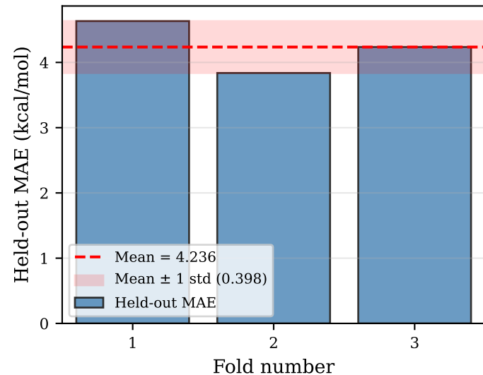
3-fold cross-validation
