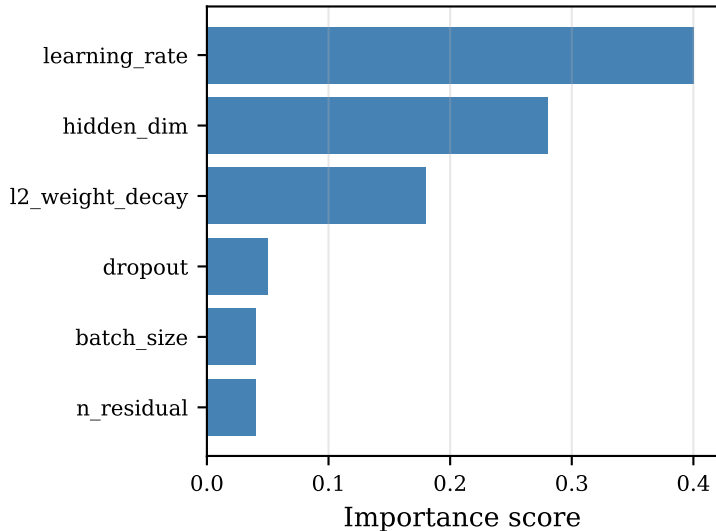
Hyperparameter importance (fANOVA)
