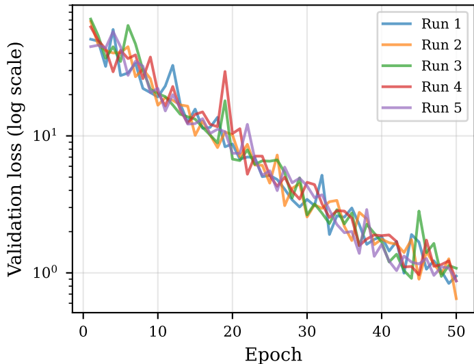
Validation learning curves (all runs)
