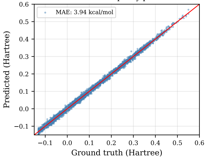
Validation parity plot
