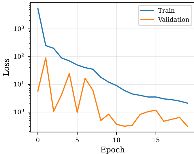
Final-model training curve
