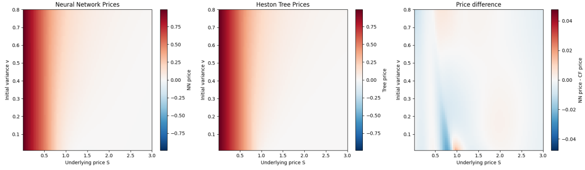
Figure 4.2 American put option prices
