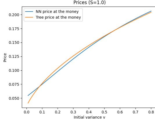
Figure 4.4 At-the-money price with varying initial variance
