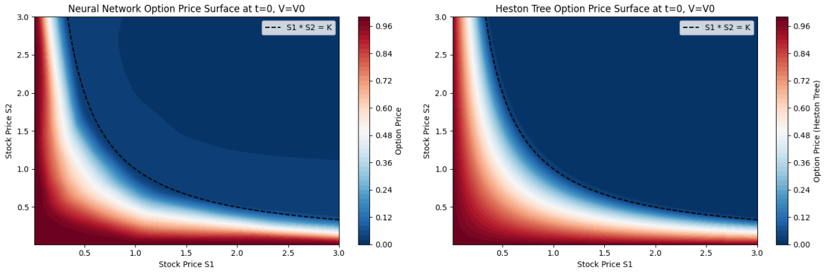
Figure 4.5 Neural network vs 1D reduction tree prices
