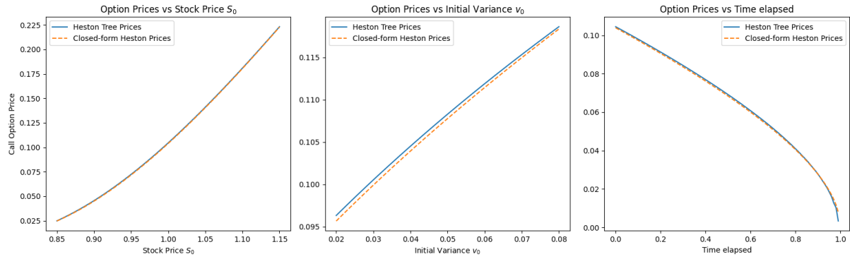
Figure 4.6 Call option prices by the Heston Tree
