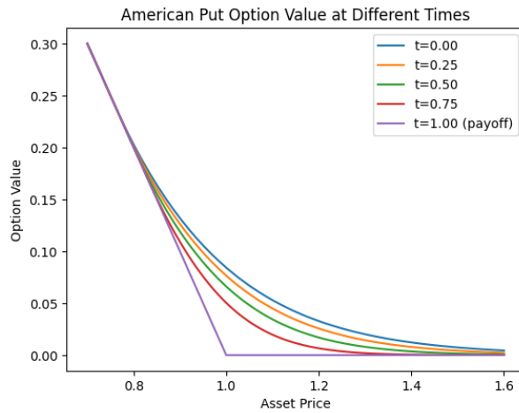
Figure 2.1 Option value on different asset prices across time
