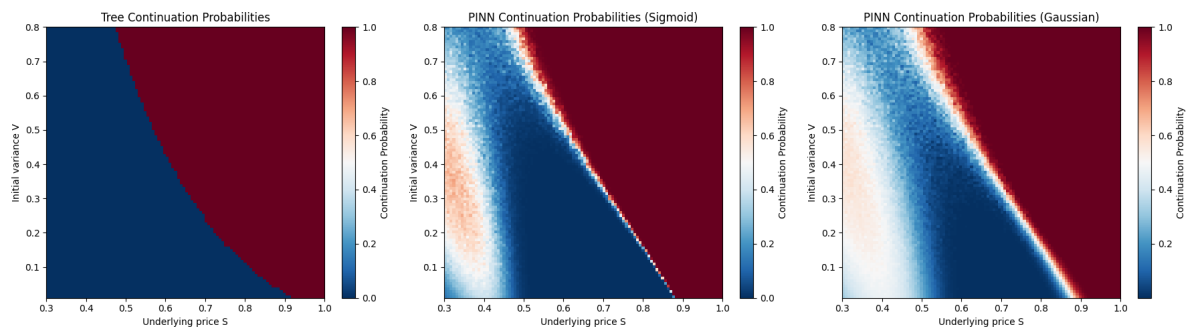
Figure 4.6 Continuation probabilities for the American put option on the S - V plane
