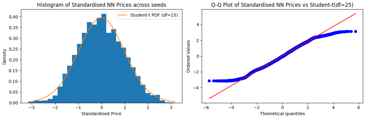
Figure 3.8 Distribution of standardised neural network price estimates across 25 runs
