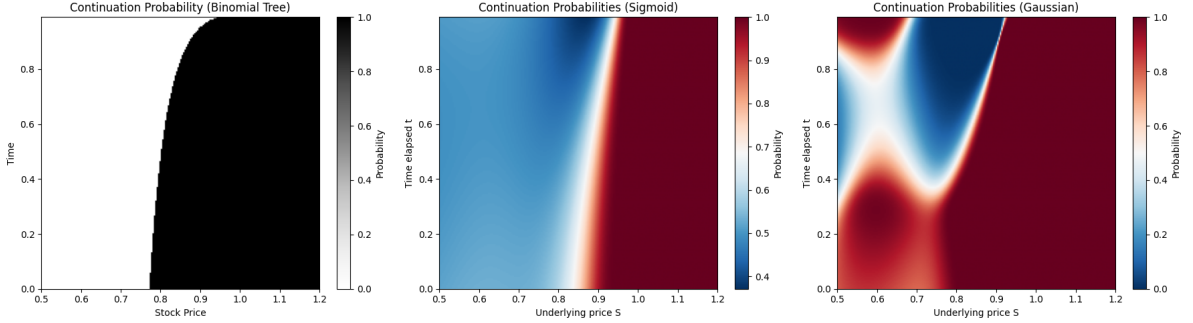
Figure 3.7 Estimated continuation probabilities from PINN for the American put option
