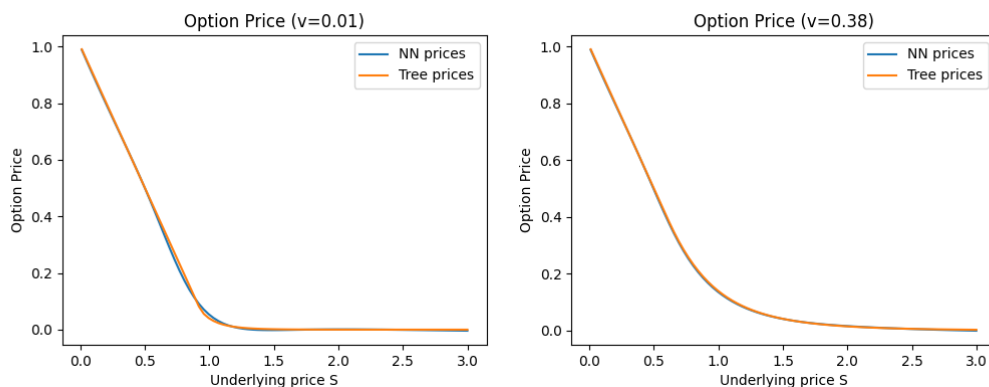
Figure 4.5 American put option prices with volatility fixed
