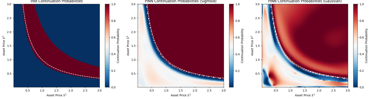
Figure 4.8 Continuation probabilities for the American put option on the S^1 - S^2 plane
