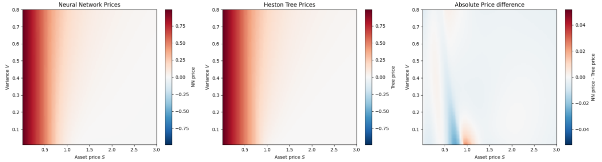
Figure 4.4 American put option prices by the PINN and the tree across S and V parameters at time t = 0
