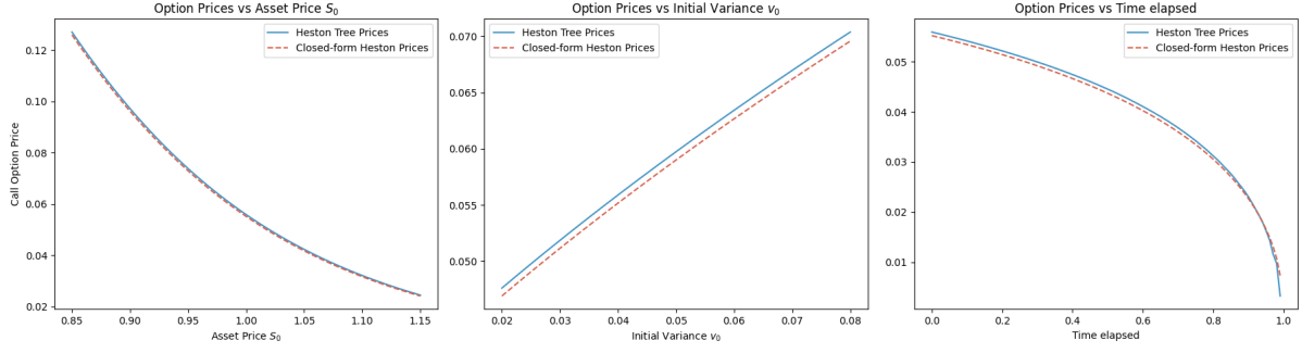
Figure 4.2 Call option prices by the Heston Tree
