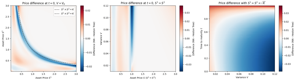
Figure 4.6 Heatmap of the difference between PINN and tree prices
