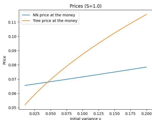
Figure 7.8 At-the-money price with varying initial variance
