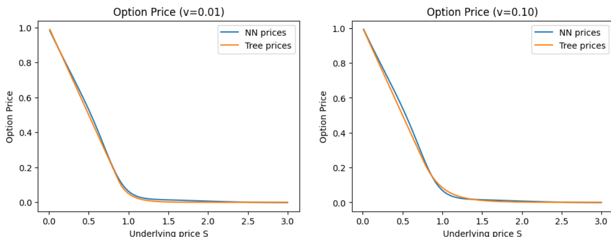
Figure 7.7 American put option prices with volatility fixed
