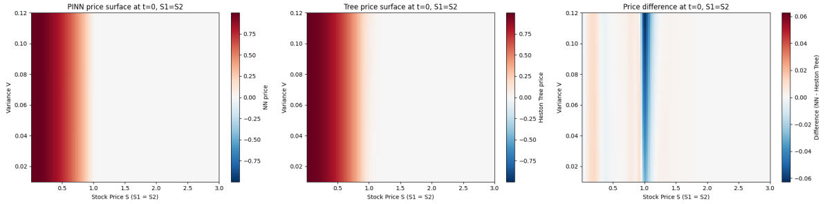
Figure 4.7 American put option prices by the PINN and the tree across S_1 and V , with t = 0 and S_1 = S_2 = \sqrt{K}
