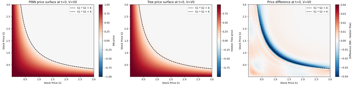
Figure 4.6 American put option prices by the PINN and the tree across S_1 and S_2 with time and variance fixed at t = 0 and V = 0.04
