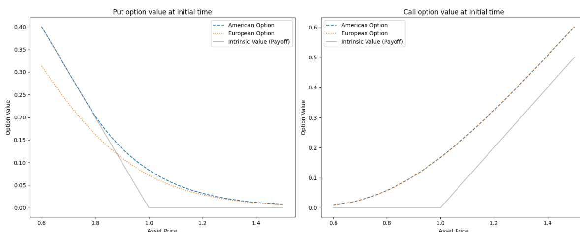
Figure 1.1 Put and Call option values at initial time
