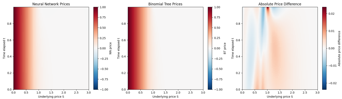
Figure 3.5 PINN vs tree price comparison for American put option
