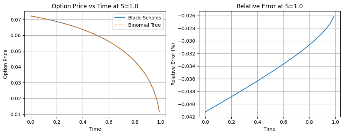
Figure 3.3 Comparison of tree and closed-form prices for European put option with varying time
