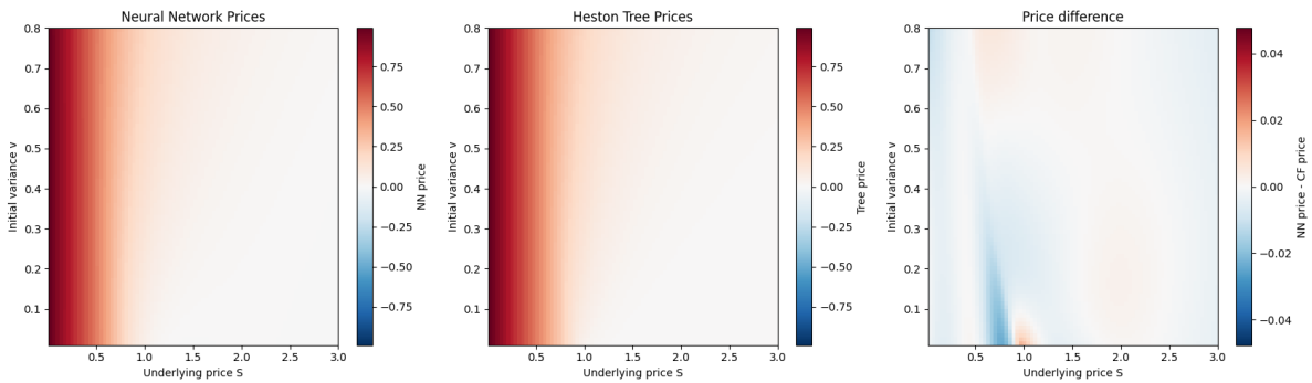
Figure 4.6 American put option prices
