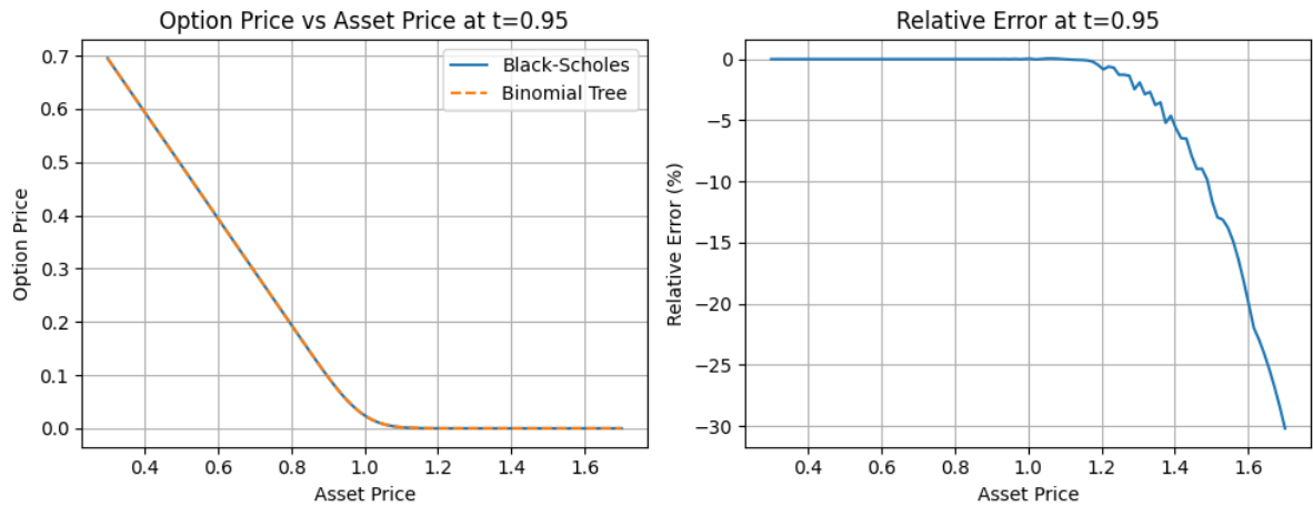
Figure 3.2 Comparison of tree and closed-form prices for European put option with varying initial asset price
