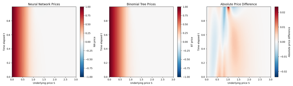
Figure 3.4 PINN vs tree price comparison for American put option
