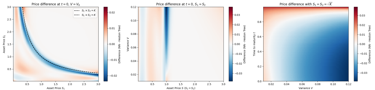
Figure 4.6 Heatmap of the difference between PINN and tree prices
