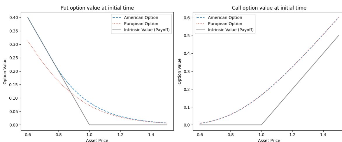
Figure 1.1 Option values (for put and call) at initial time
