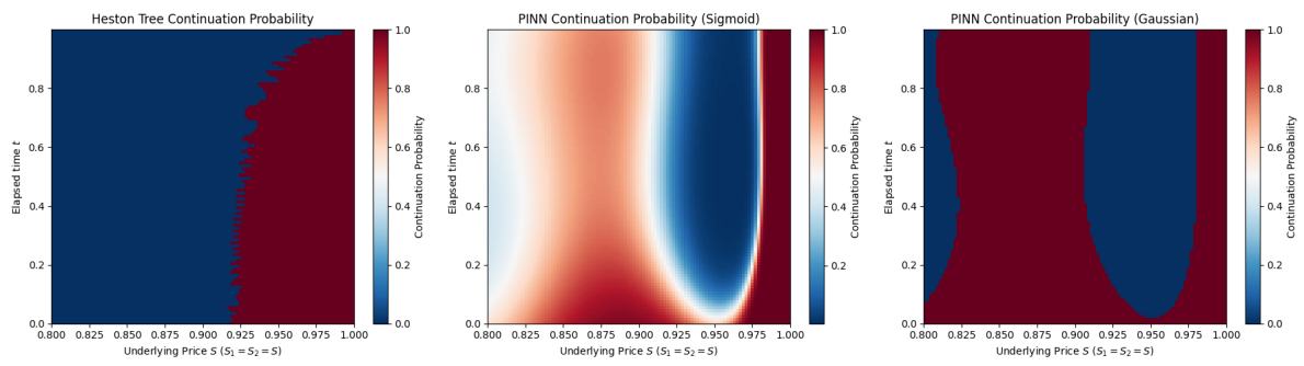
Figure 4.9 Continuation probabilities for the American put option on the S - t plane
