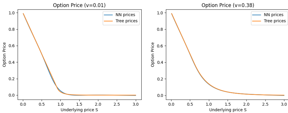
Figure 4.7 American put option prices with volatility fixed
