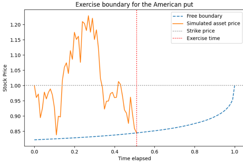
Figure 1.1 Exercise boundary for the American put
